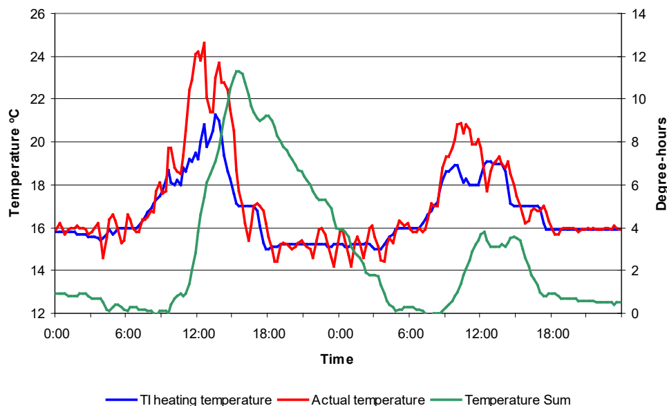
Figure 3 – TI control
