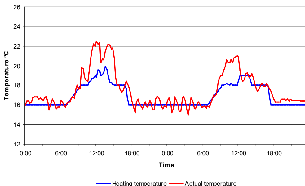
Figure 2 – Conventional control
